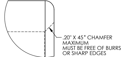
OPTIONAL SHANK-END CONFIGURATION
