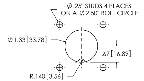
TANK HOLE DIMENSION (EXTERNAL MOUNTING)
