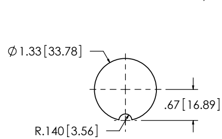
TANK HOLE DIMENSION (INTERNAL MOUNTING)
